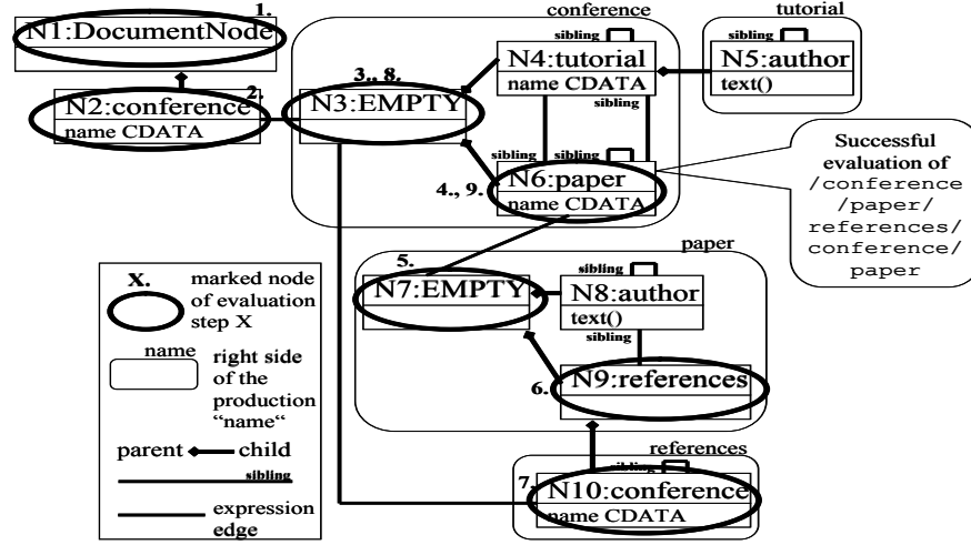
Fig. 9. Ordered schema graph with marked nodes according to the query conference/paper/references/conference/paper
