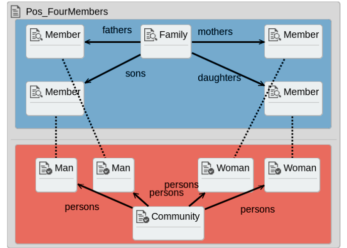
Figure 3: Pos_FourMembers contract, representing the informal statement “A Family with a father, mother, son and daughter should always produce two Man and two Woman elements connected to a Community”
