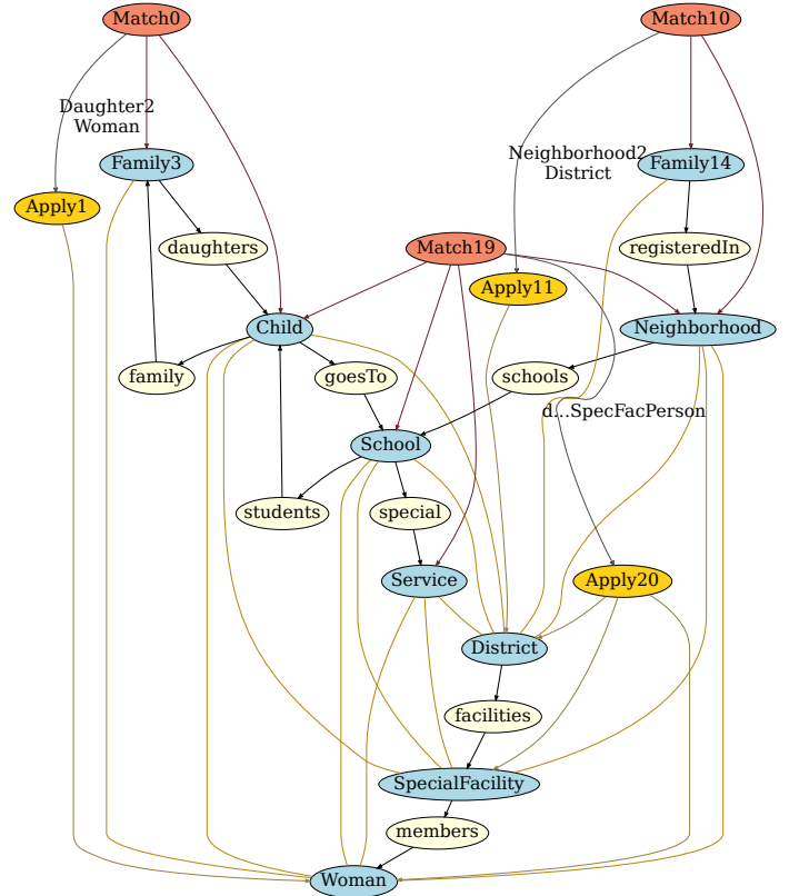
Figure 8: An unintuitive visualization of a path condition that fails to satisfy the SchoolOrdFac contract.
