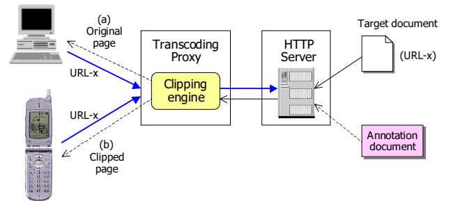
Figure 3: Overview of an annotation-based transcoding
