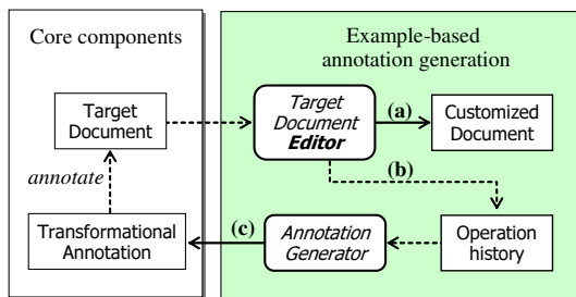
Figure 2: Tool configuration for transformational annotation by example
