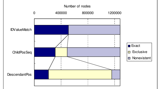
Figure 12: Number of nodes with detailed distinction of pointing status
