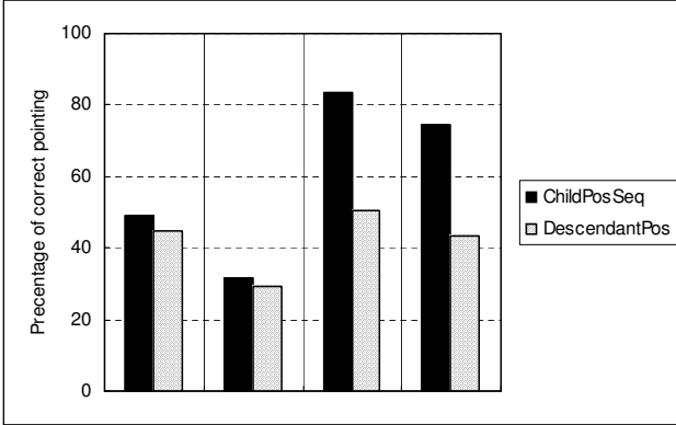
Figure 11: Percentage of correctly pointed nodes for each XPath expression
