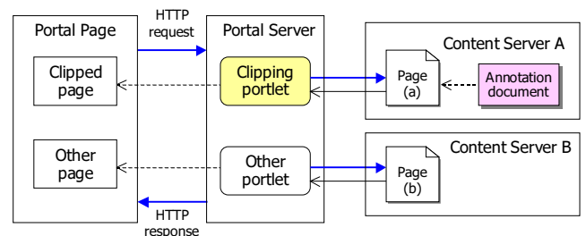
Figure 6: Creation of a portal page with annotation-based clipping portlet
