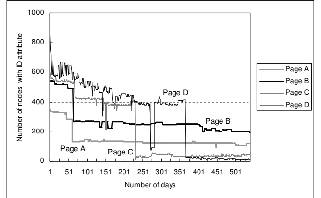
Figure 9: Number of nodes with ID attributes during the observation period
