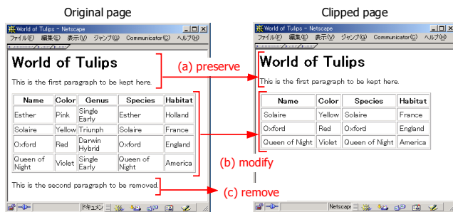
Figure 4: Simple example of an HTML page clipping
