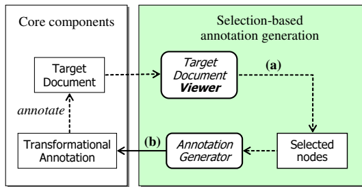
Figure 1: Tool configuration for transformational annotation by selection
