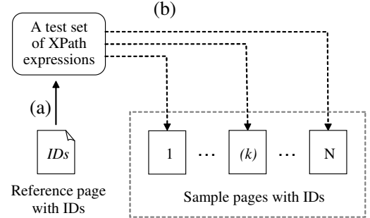
Figure 10: Process of testing XPath expressions
