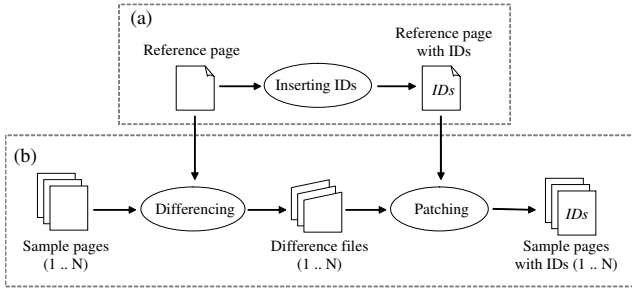
Figure 8: Process of node ID insertion
