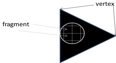
Figure 1 Shader Structure
