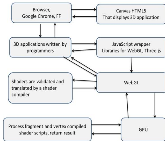
Figure 2 WebGL Stack
