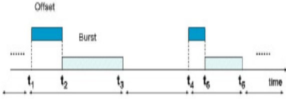
Fig. 3. JIT reservation protocol
