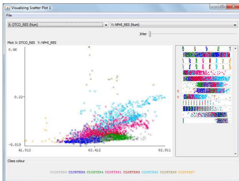
Fig. 4. Scatter plot
