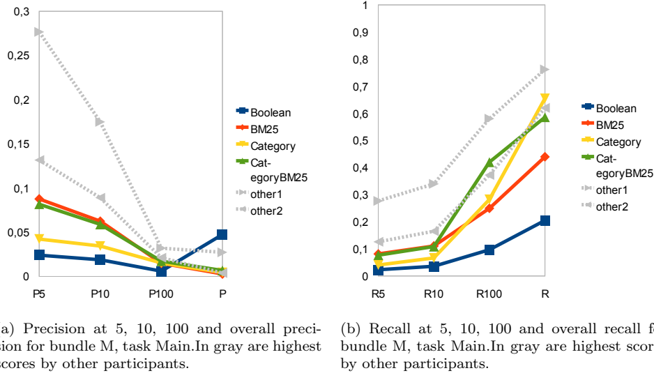
Figure 3: Precision and recall curves for our 4 submissions, for comparison two runs from other participants have been added. (source: [6], Table 9)
