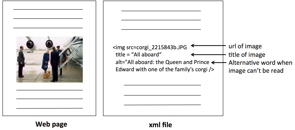
Fig. 2. Attributes of image tag.
