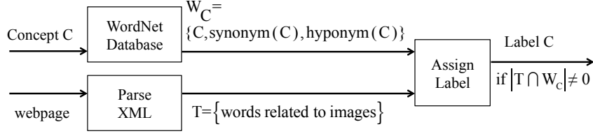
Fig. 1. Pipeline of label assignment.
