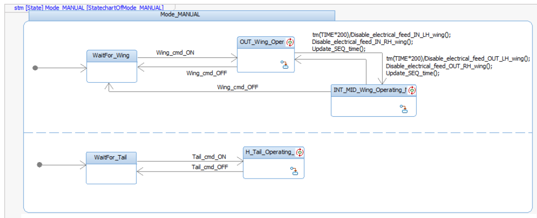
Figure 3. State Machine diagram – Manual Mode
