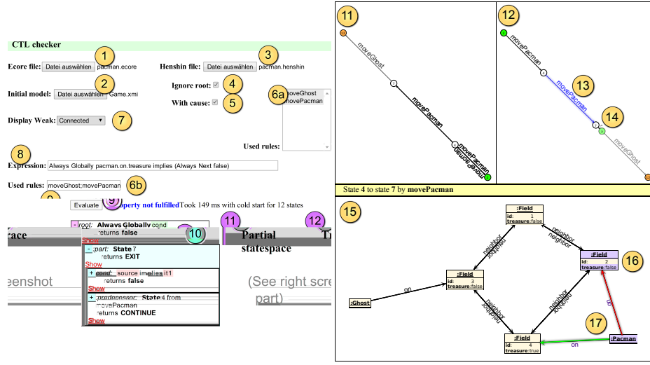
Fig. 4: The MocoCL state space and model view
