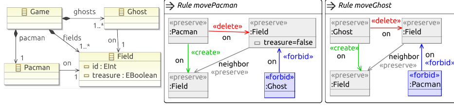
Fig. 3: Ecore model and HENSHIN transformation rules
