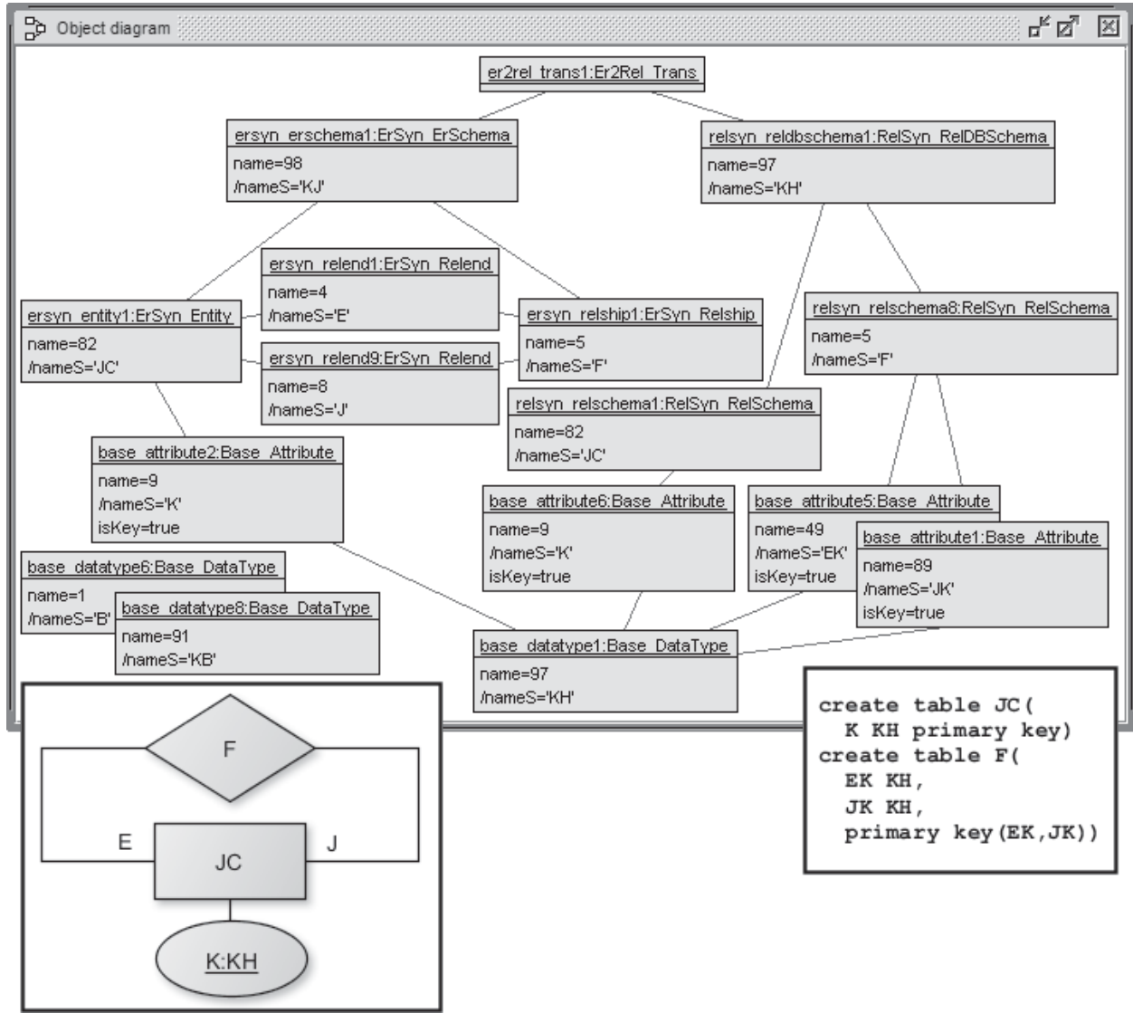
Fig. 6. Generated proof example for class instantiability.
