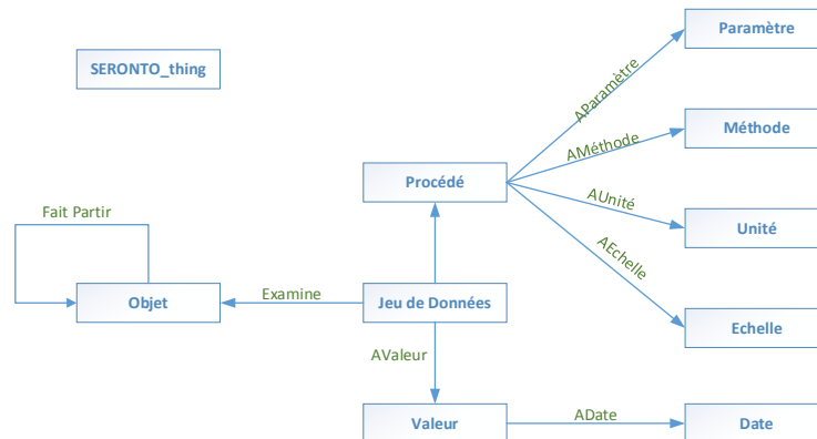
Figure 1 : Concepts de base de SERONTO
