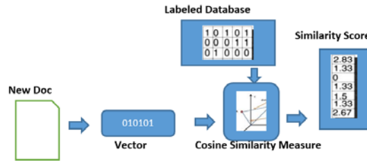
Fig. 1. Computing Similarity score
