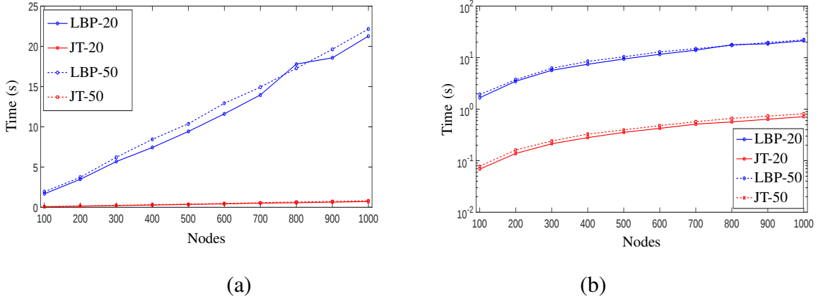
Fig. 2. Time to compute the posterior probabilities for LBP, and the JT algorithm for cluster networks with different cluster sizes ( n_c = 20 and 50 ) and m = 3 for the dynamic analysis of the BAGs (when we observe evidence of attack at 3 random nodes): (a) Time in natural scale; (b) Time in logarithmic scale.
