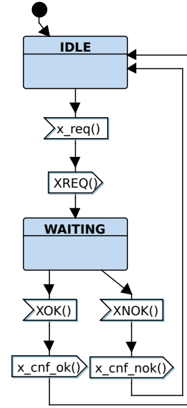
Fig. 6. Protocol Machine for the Requester
