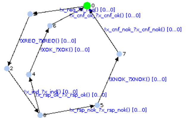
Fig. 8. Reachability Graph
