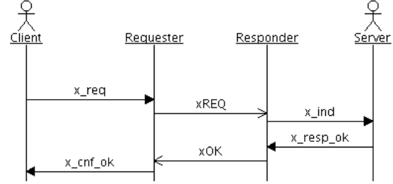
Fig. 4. Protocol Scenario (successful request)
