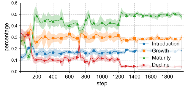
Figure 5: Percentage of impressions allocated to different stages.
