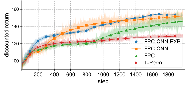
Figure 4: Performance Comparison between algorithms
