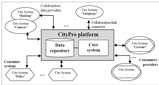
Fig. 1. CityPro's target system
