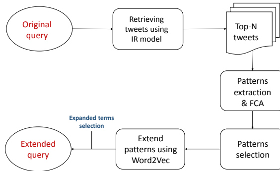
Fig. 1. Overview of the proposed query expansion approach.
