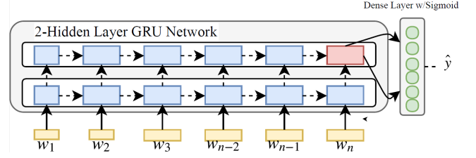
Figure 1: GRU-based Ensemble Architecture (red corresponds to the last hidden state vector that outputs embedding for both in-domain and large pretrained embedding inputs)
