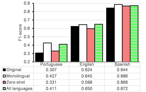
Figure 4. Comparison of the performances for Monolingual, Zero-shot and One-shot
