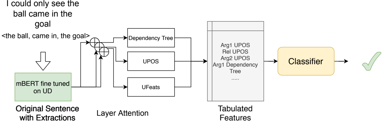
Figure 1. Architecture overview
