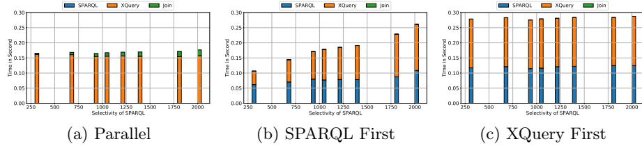
(a) Parallel (b) SPARQL First (c) XQuery First Fig. 4: Detail of Execution Time in L.S. Scenario with XQuery Selectivity of 660
