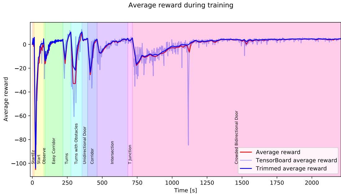
Figure 4: Average reward throughout training.
