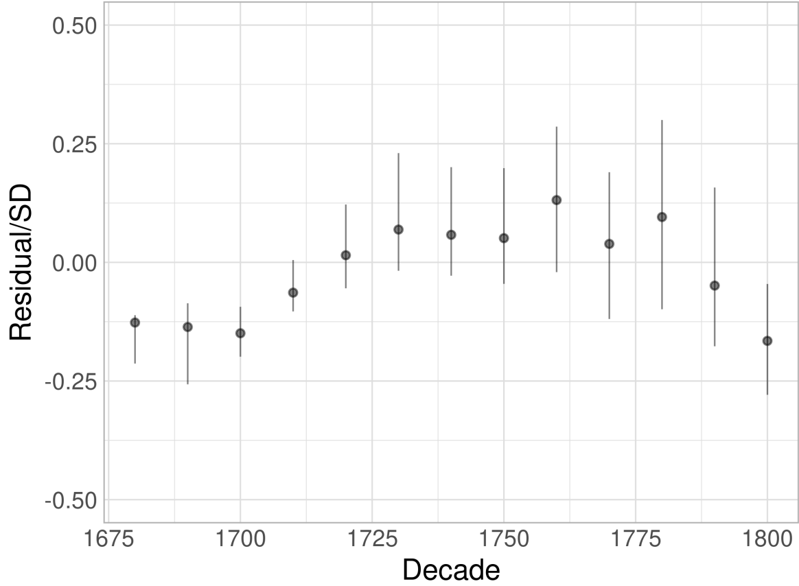
Figure 3: The median residuals of the test data for roughly average sized (standardised plates and paper \pm 0.5 SD from Zero) print products 1680-1800 in London. Confidence Interval from 1st quantile of residuals to the 3rd quantile. Standardised by dividing with the standard deviation of the test data which was used to make this figure.
