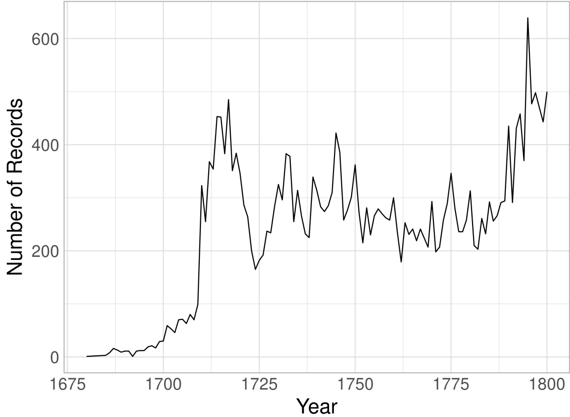
Figure 1: The observations used in this article, 28251 in total, by publication year. Most of the price information is from the eighteenth century.
