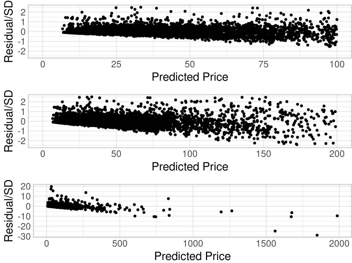
Figure 2: Predicted price (mean of the posterior predictive distribution) and residuals divided with the standard deviation of the test data. The visualisations were done with different X and Y axis to demonstrate the importance of variation by price and the effect of outliers. 814 Observations of the total test data are missing from the top panel and 243 from the middle panel.
