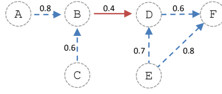
Figure 2: Similarity in the Bipolar Argumentation Framework (Fig 1)
