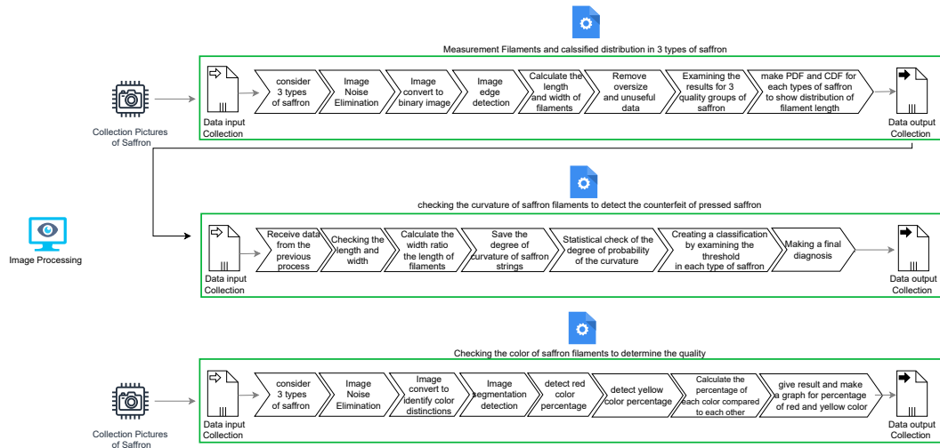
Figure 6: Image processing
