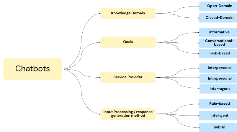
Figure 1: Chatbots classification
