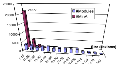
Figure 2: Module and MinA size distribution.
