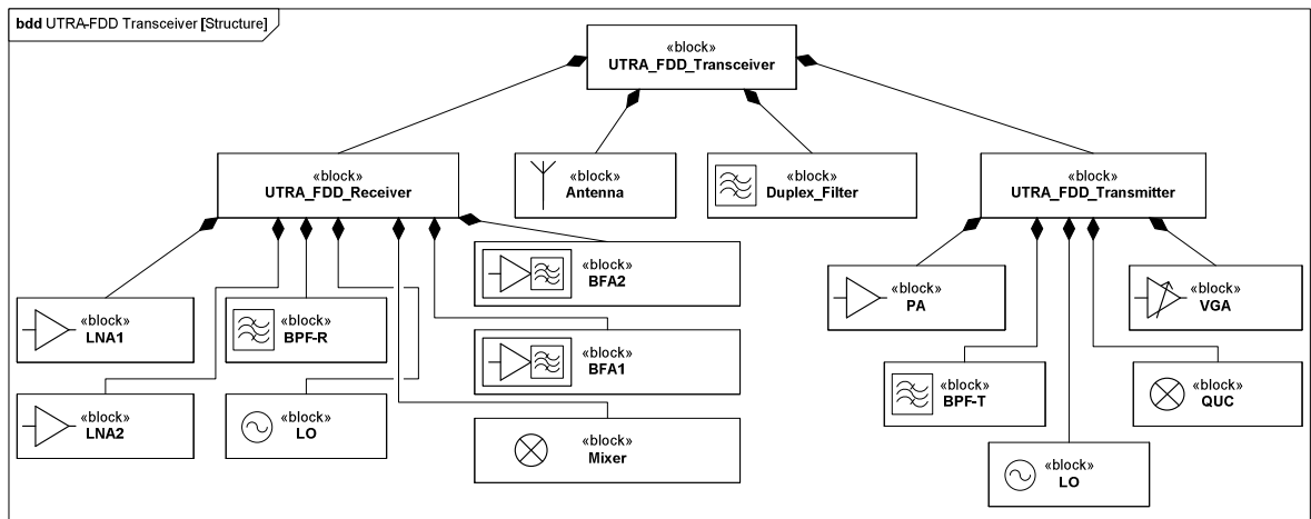
Fig. 10. An example of block definition diagram incorporating notations belonging to RF engineering domain.
