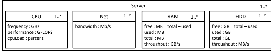
(a) CCM Structure Model for Hardware Landscapes.
