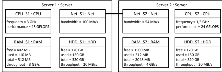
(a) CCM Structure Model for Hardware Landscapes.
