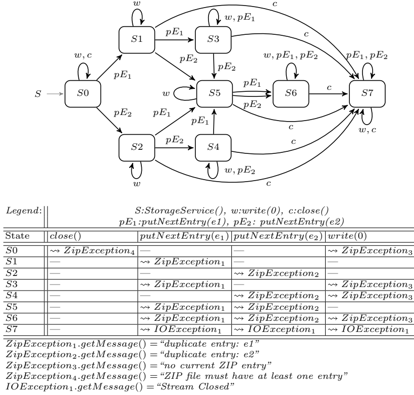
Fig. 1. A BEM of the STORAGESERVICE component
