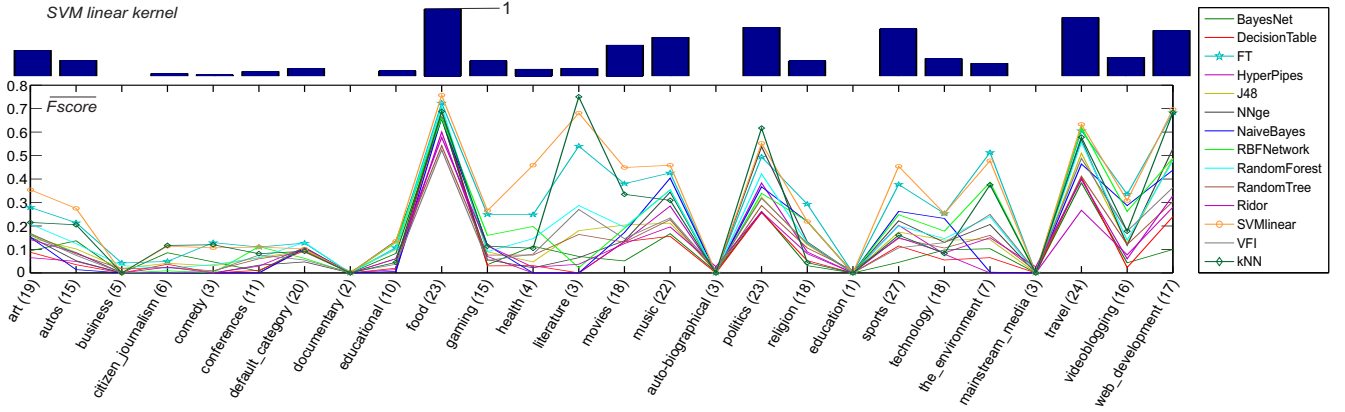
Figure 1: Average F_{score} achieved using all audio-visual descriptors and genre classification "performance" for the best run, i.e. SVM with linear kernel (graph on top).
